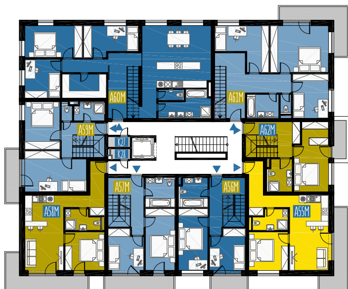
8.NP / 8TH FLOOR
